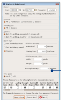
Figure 8. Customizable reports
